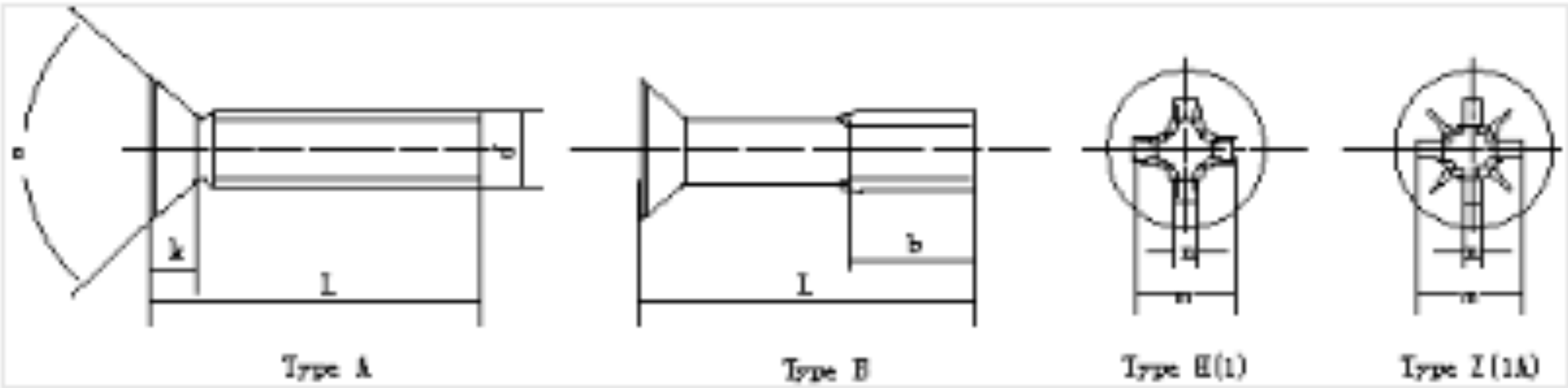
DIN 965 CROSS RECESSED COUNTERSUNK FLAT HEAD SCREWS Thread Size : M3-M10 Length(L): 6-100mm
