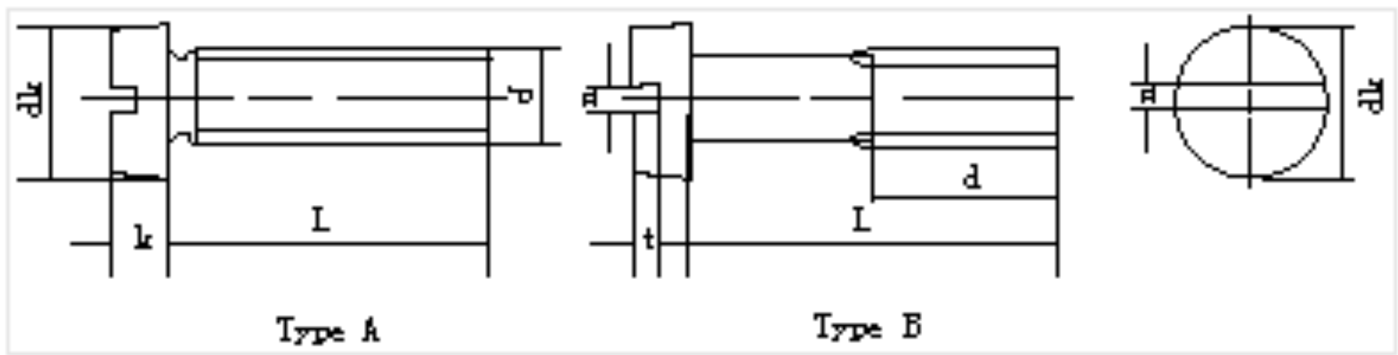
DIN 965 CROSS RECESSED COUNTERSUNK FLAT HEAD SCREWS Thread Size : M3-M10 Length(L): 6-100mm
